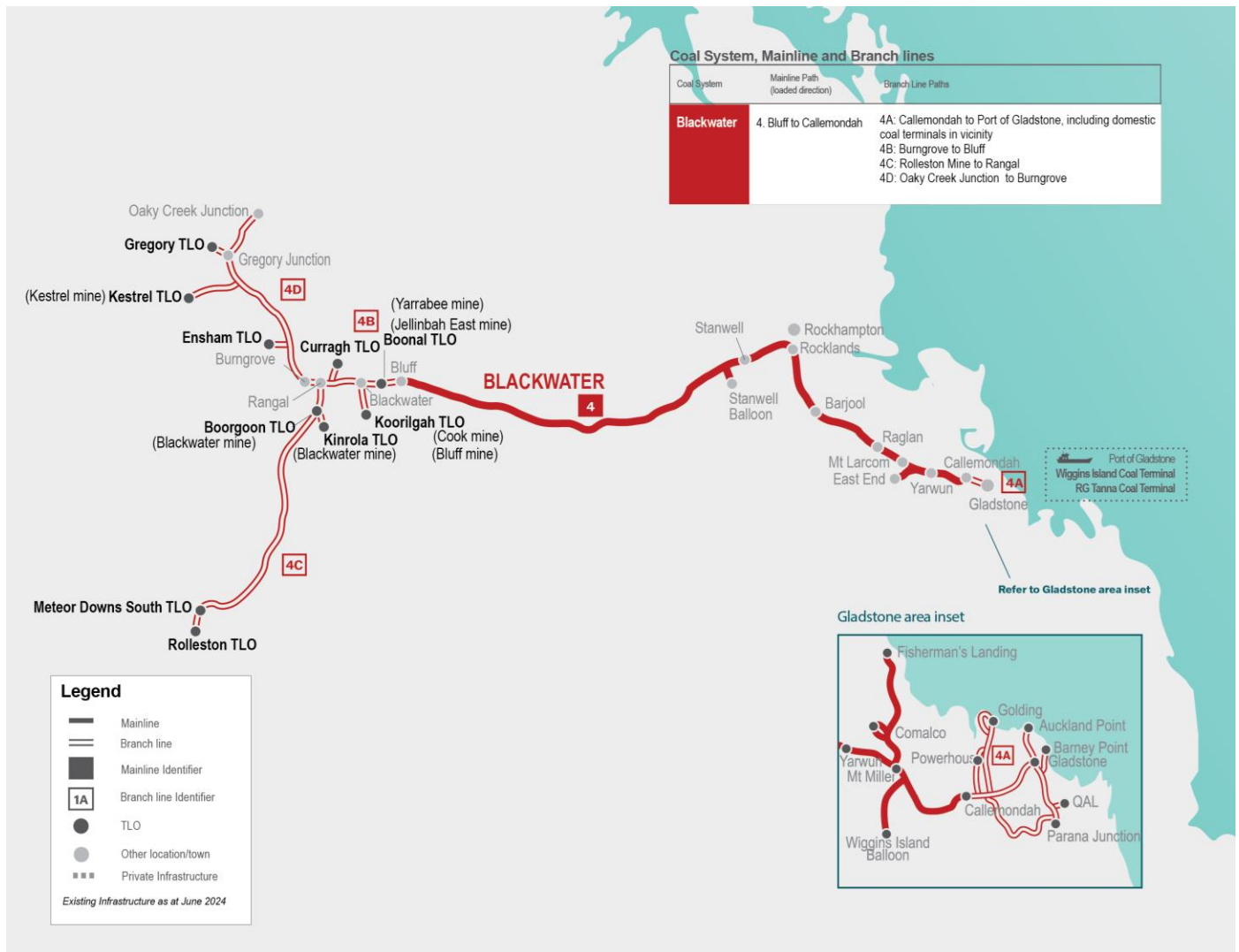
Figure 31 - Blackwater system
