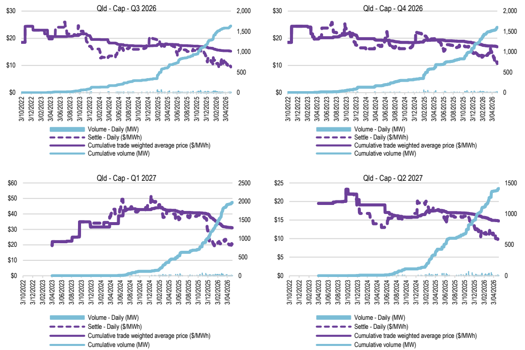
Figure 4.5 Time series of trade volume and price – ASX Energy $300 cap futures - Queensland
