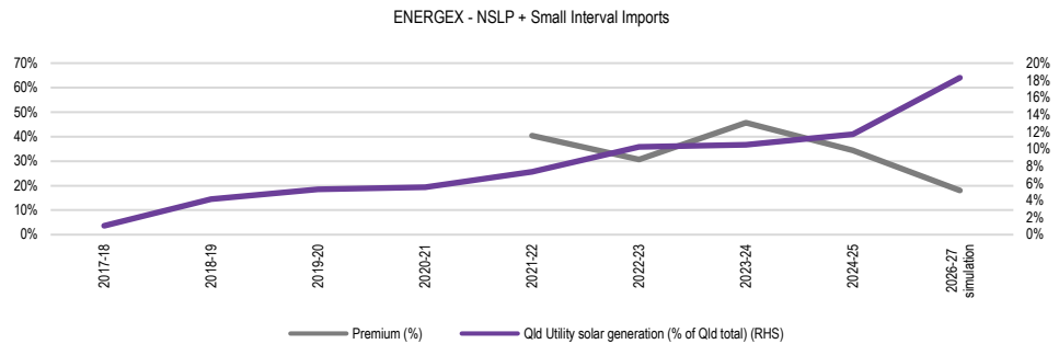
Figure 4.10 Simulated annual DWP for NSLP and Interval meter demand as a percentage premium of annual TWP for 2026-27 compared with range of actual outcomes in past years, and market share of utility scale solar (%)
