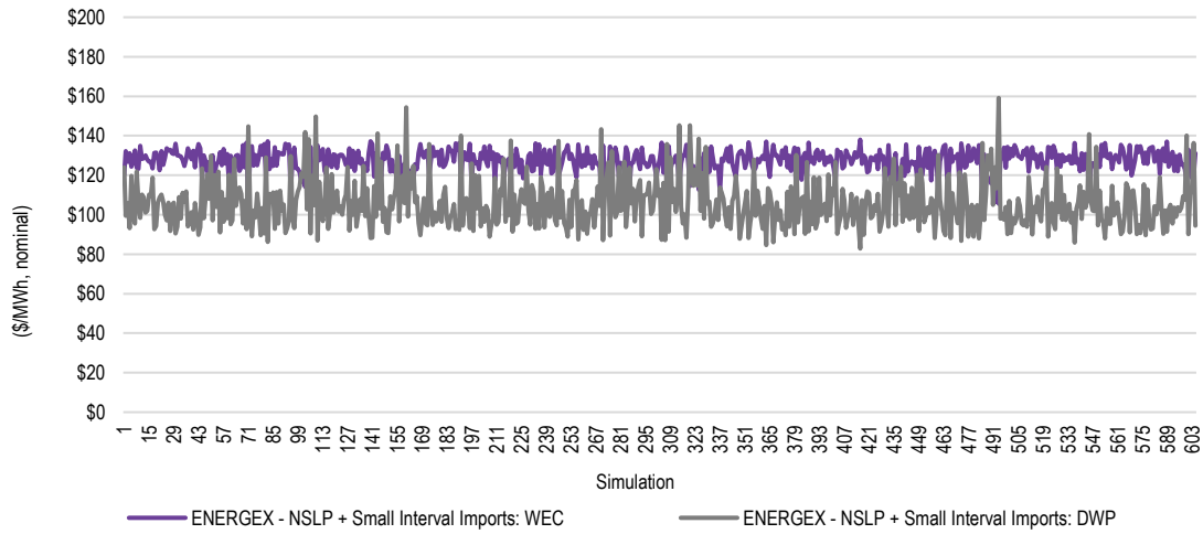
Figure 4.12 Annual WEC and DWP ($/MWh, nominal) for the Energex NSLP + small interval meter demands for the 605 simulations – 2026-27
