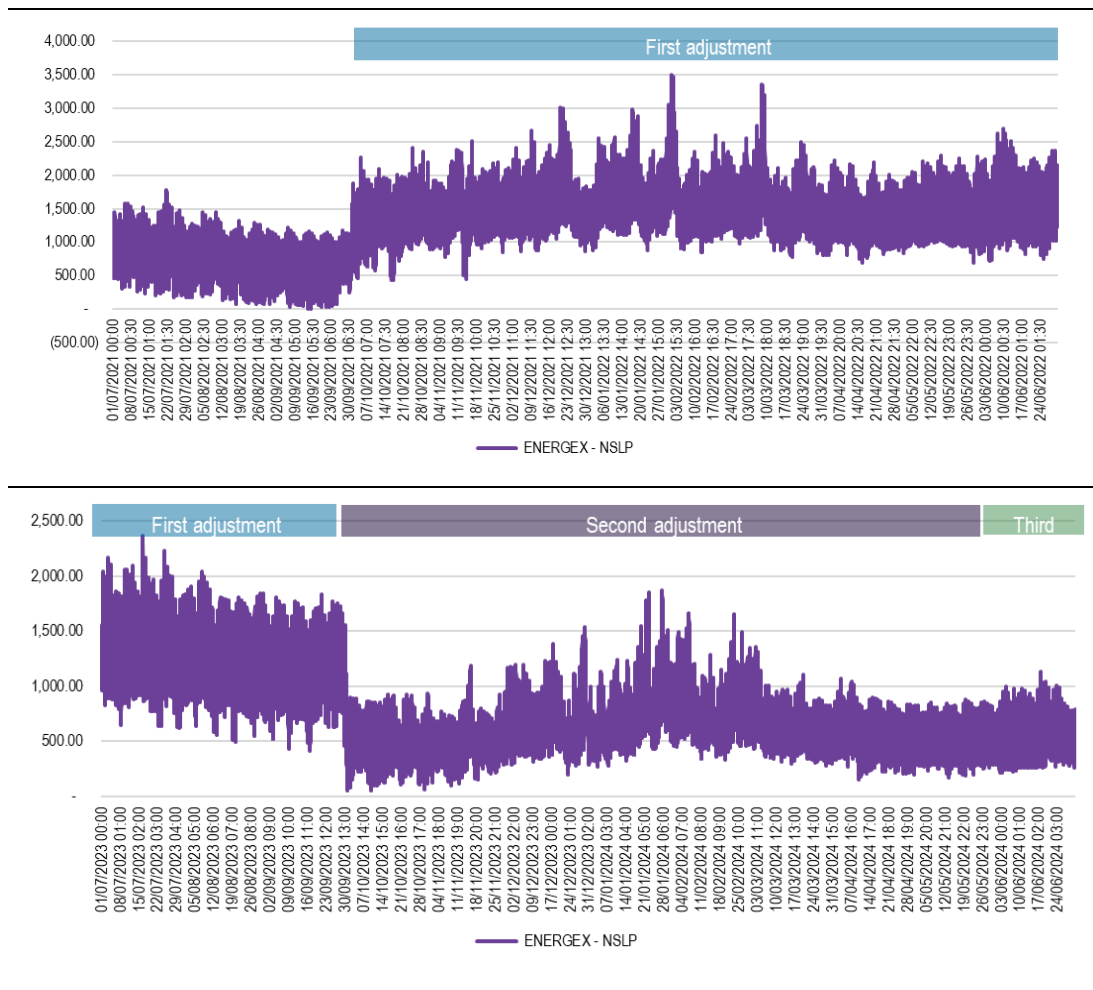
Figure 2.4 Energex NSLP (MW) – July 2021 to June 2024
