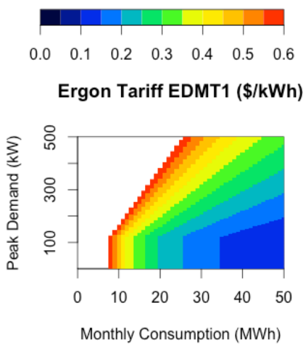
Figure 7. Ergon Tariff EDMT1 Average Price (Threshold Demand 120kW)
