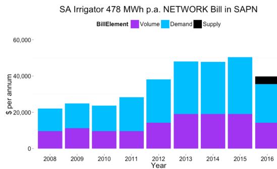
Figure 28. SA Irrigator 478 MWh p.a. network average price
