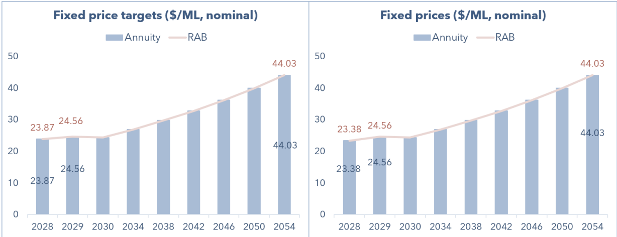
Figure 4: Fixed price targets and prices – Upper Condomine – North Branch – Risk A ($/ML)
