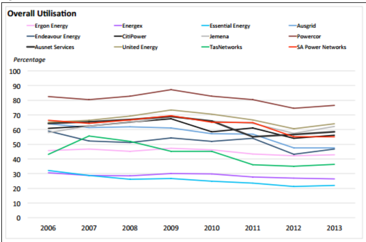
Figure 6: Network utilisation
