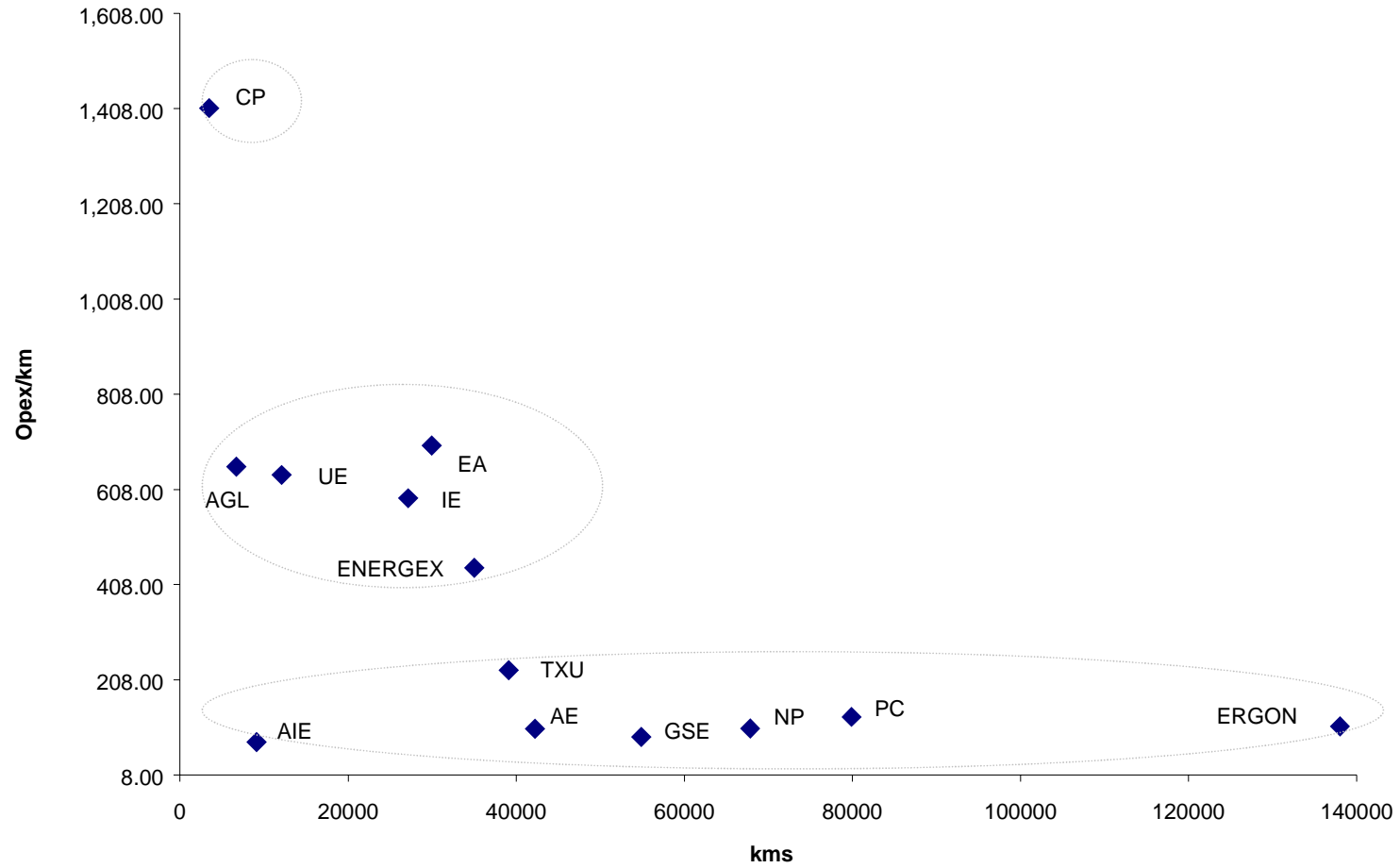
Figure 7: Opex/km and Km line length
