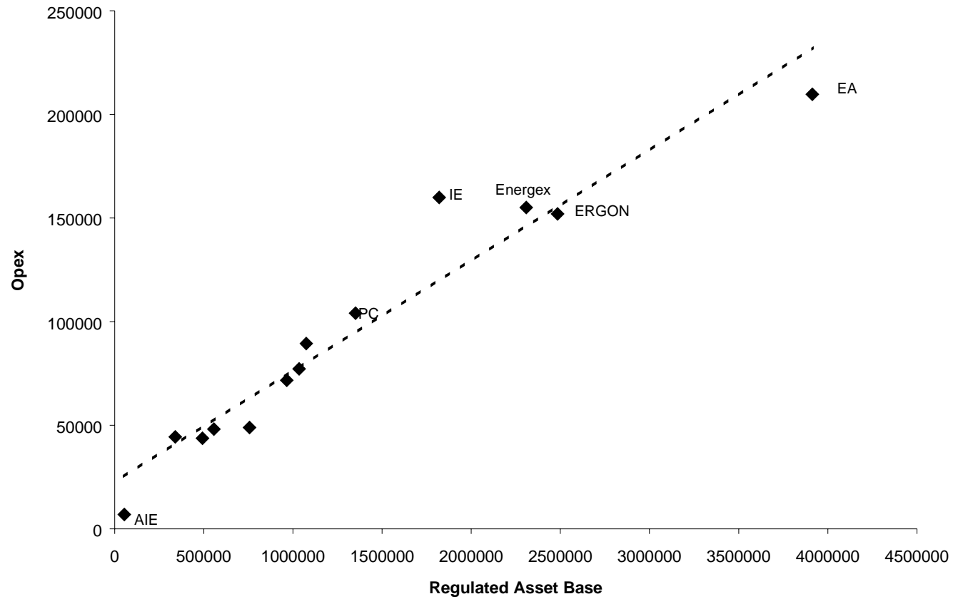
Figure 17: O&M costs and regulated asset base
