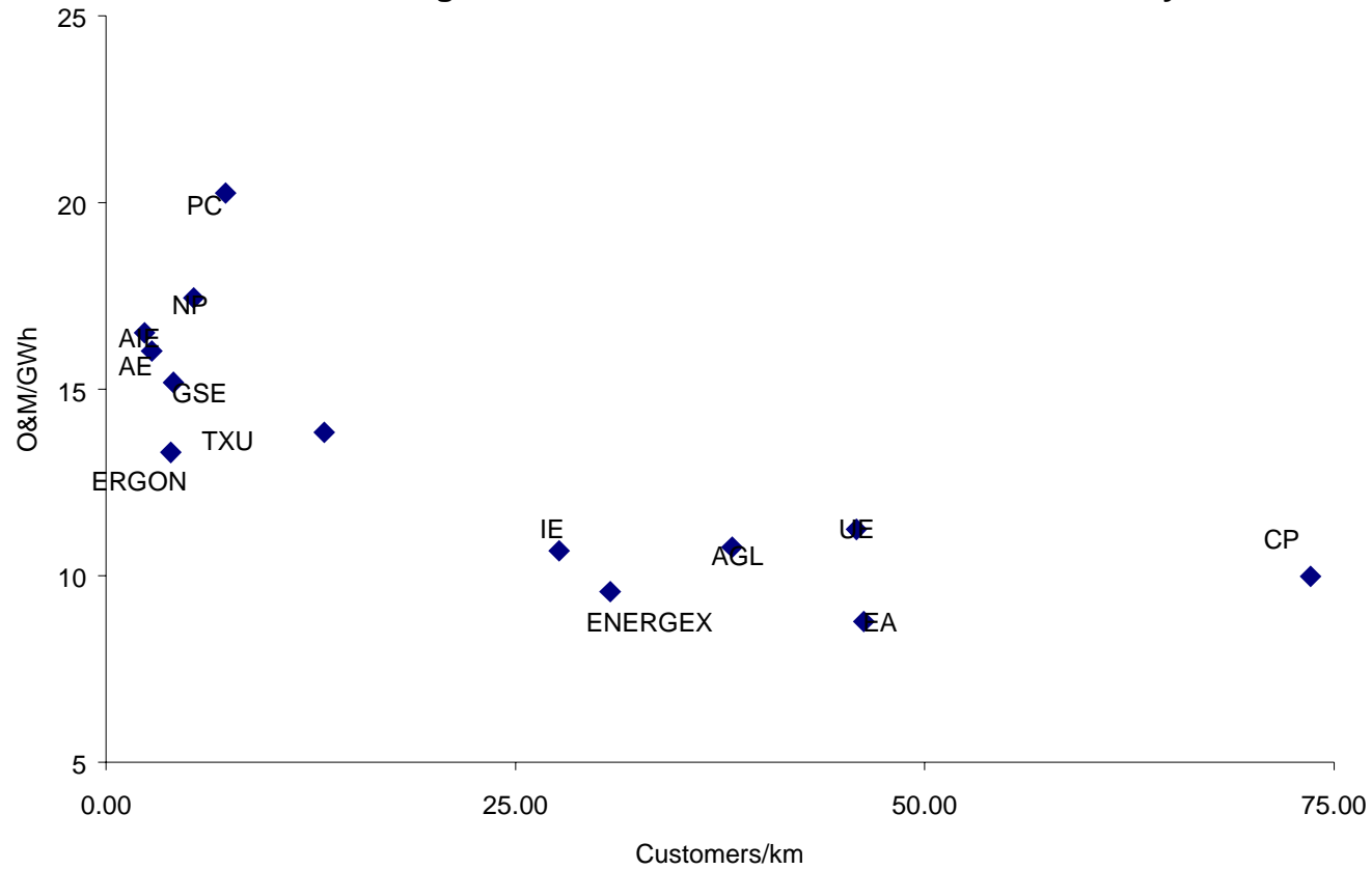
Figure 13: O&M Unit costs and Customer Density
