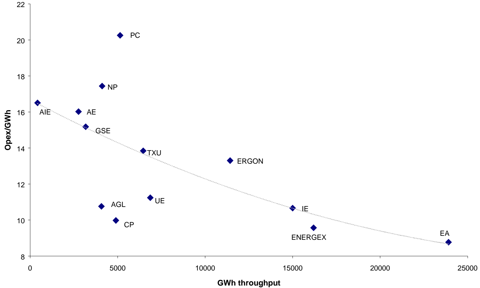
Figure 5: Opex/GWh and GWh throughput
