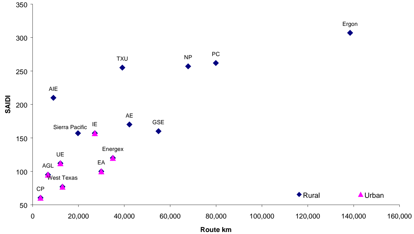
Figure 18: Route km v SAIDI, Rural and Urban DBs
