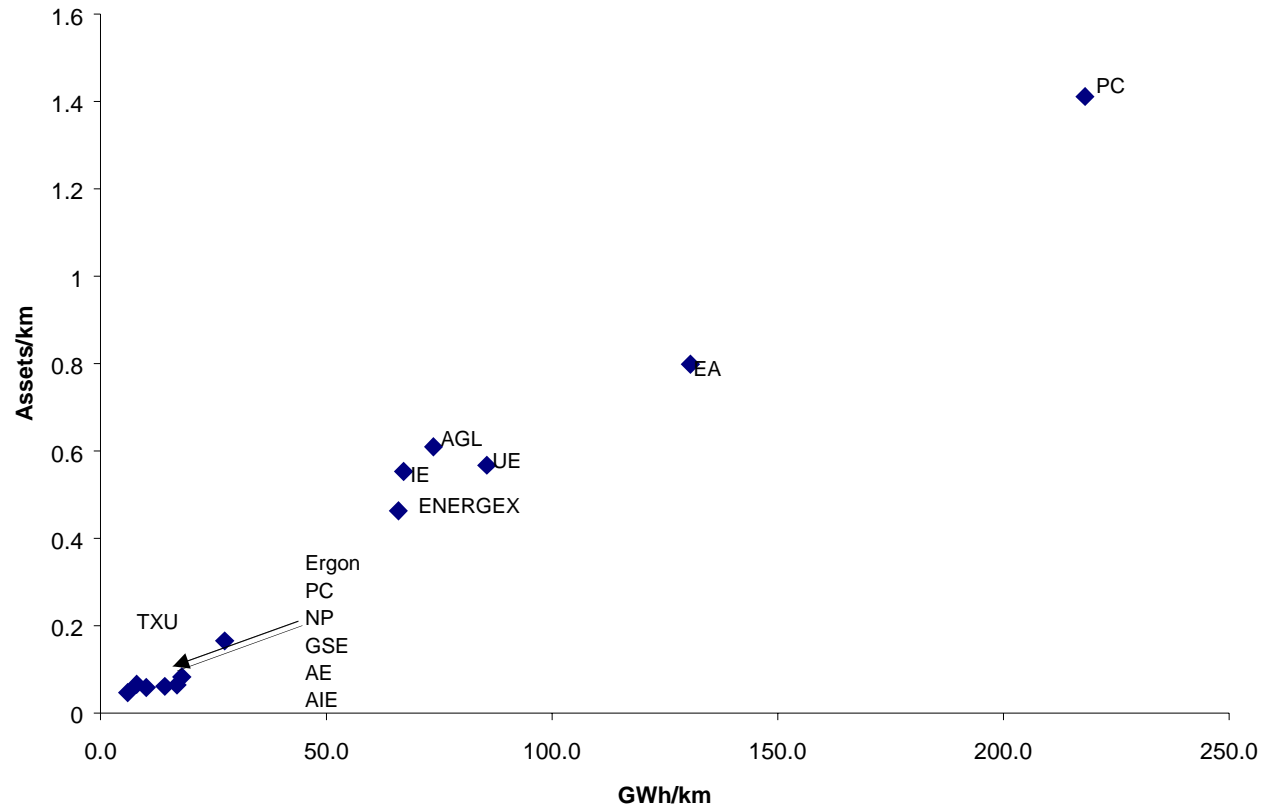
Figure 16: Assets/km and Energy density (GWh/km)
